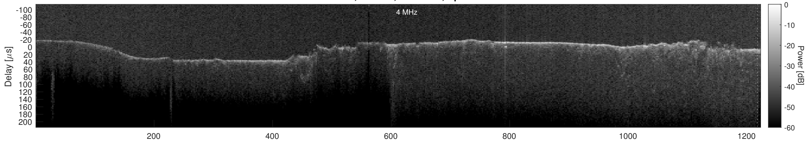
Orbit 18771, Cluttergram
