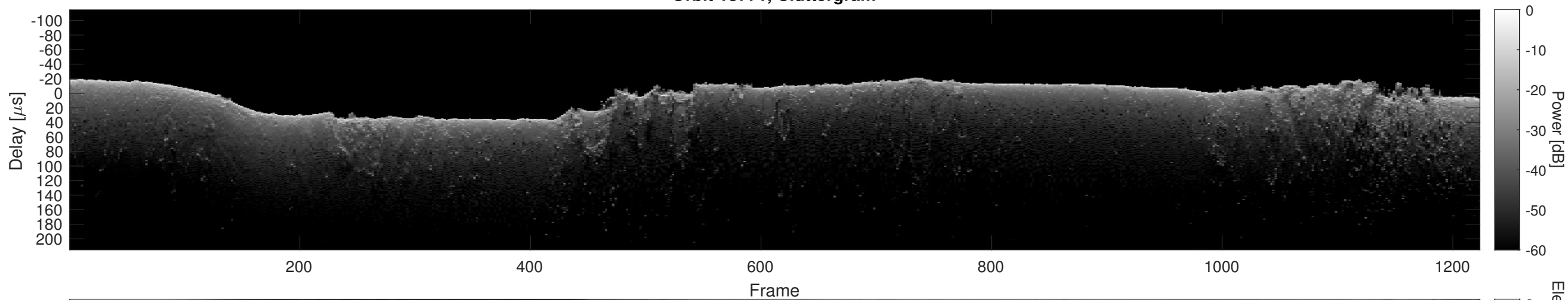
Orbit 18771, Cluttergram
