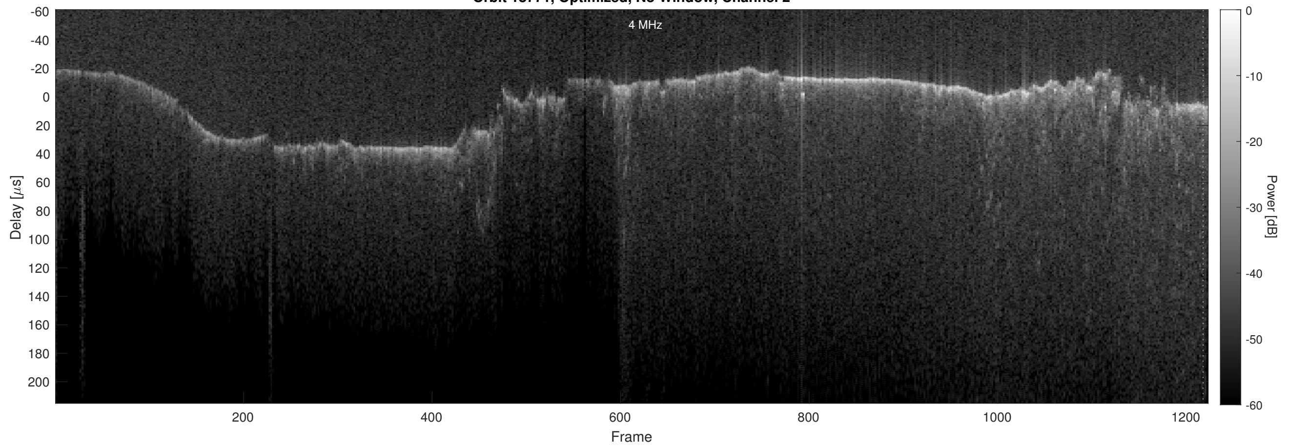
Orbit 18771, Optimized, No Window, Channel 2
