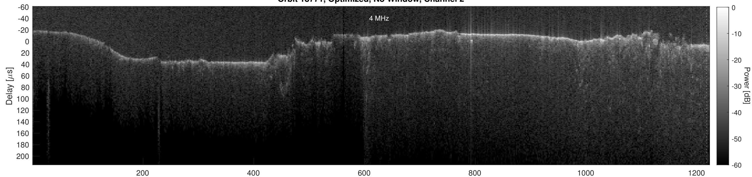
Orbit 18771, Cluttergram
