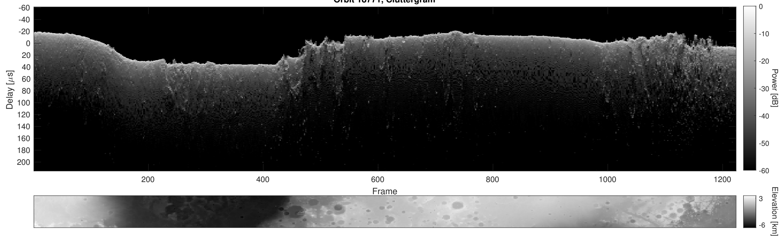
Orbit 18771, Cluttergram
