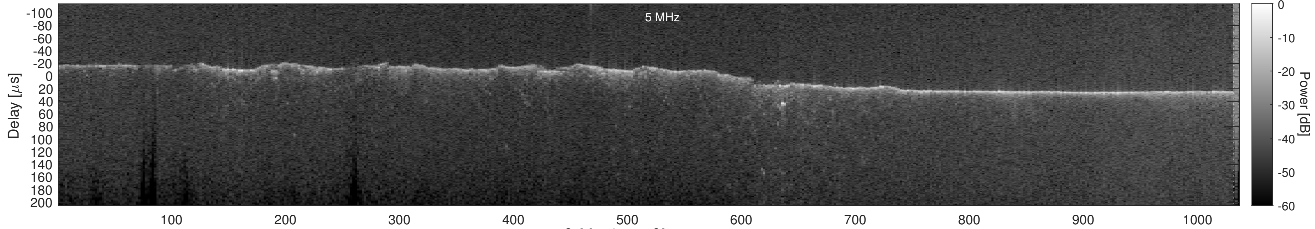
Orbit 18774, Cluttergram
