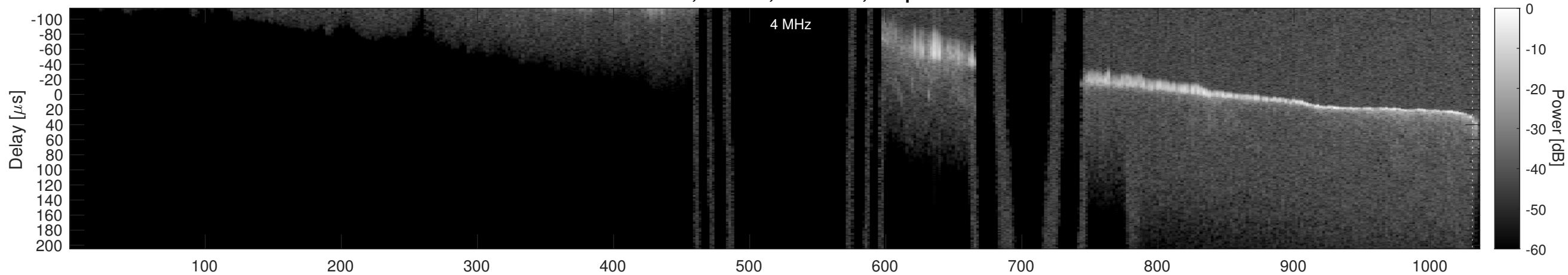
Orbit 18774, Window, Channel 2, Optimized
