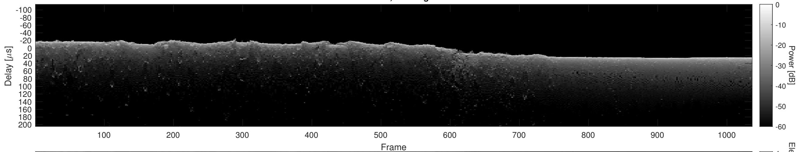
Orbit 18774, Cluttergram
