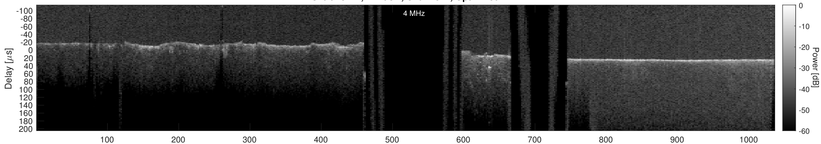
Orbit 18774, Cluttergram
