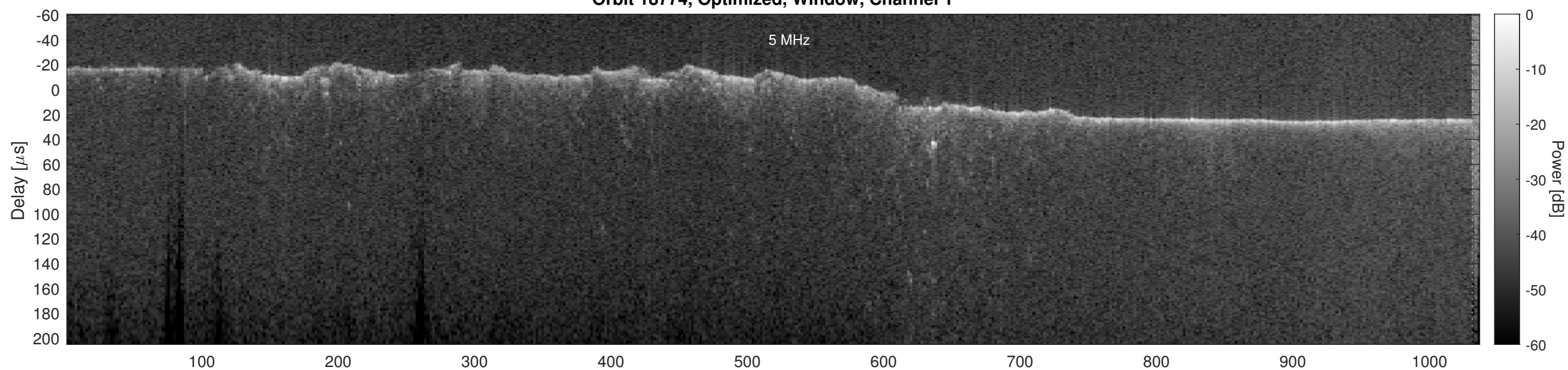
Orbit 18774, Optimized, Window, Channel 2
