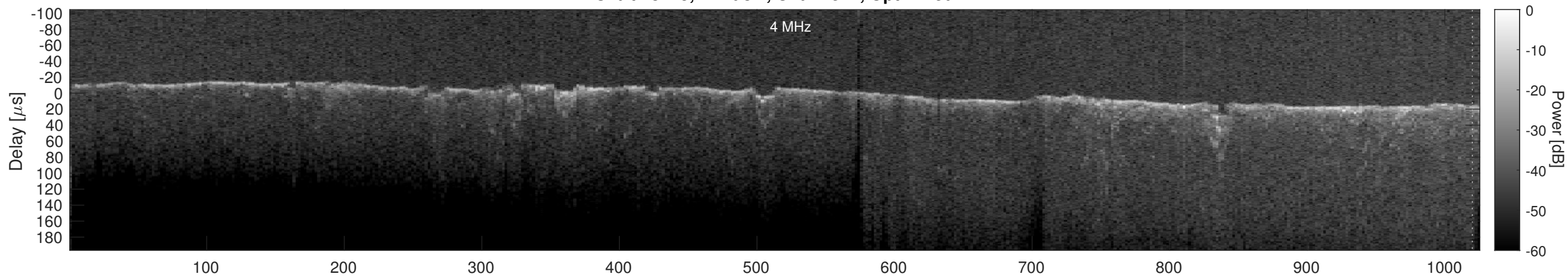
Orbit 18775, Cluttergram
