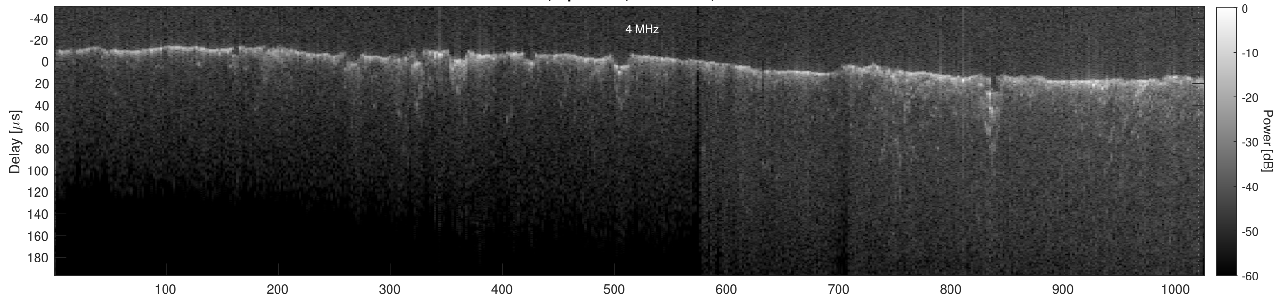
Orbit 18775, Cluttergram
