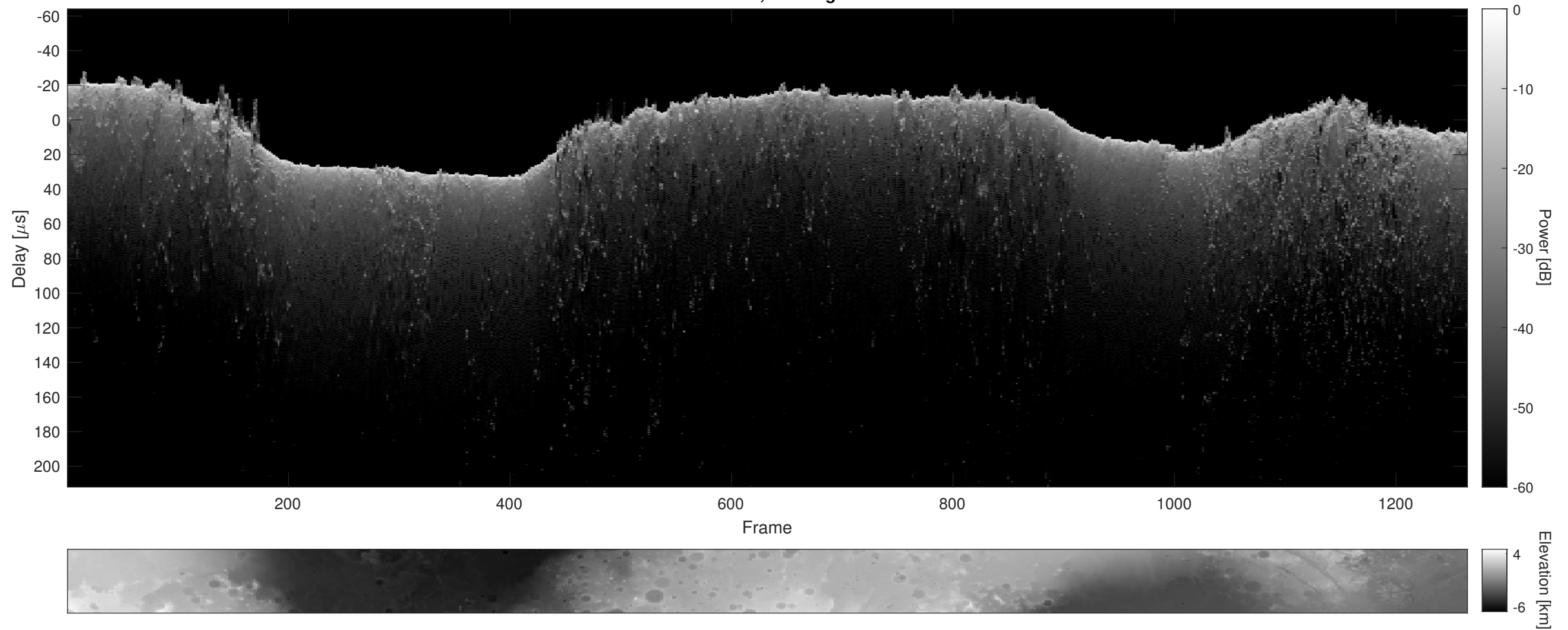
Orbit 18778, Cluttergram
