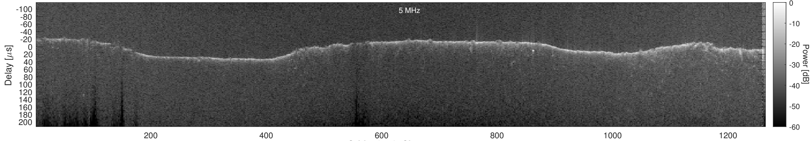
Orbit 18778, Cluttergram
