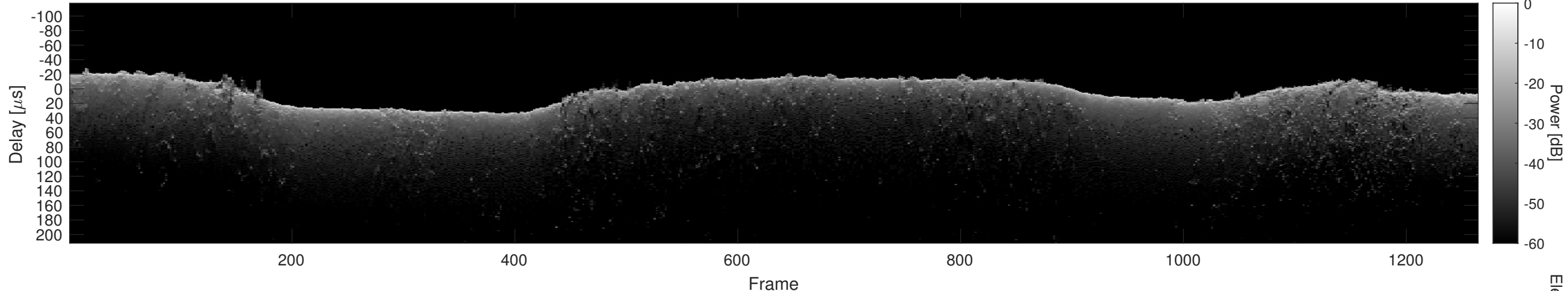
Orbit 18778, Cluttergram
