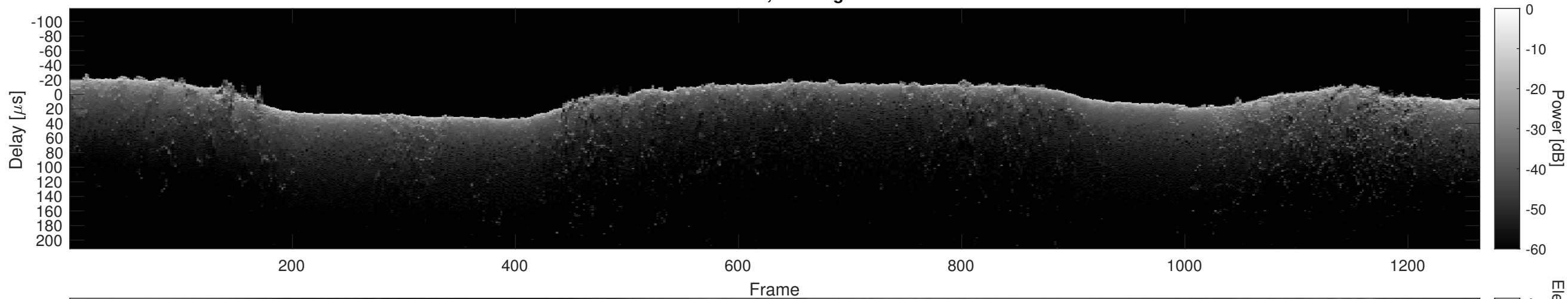
Orbit 18778, Cluttergram
