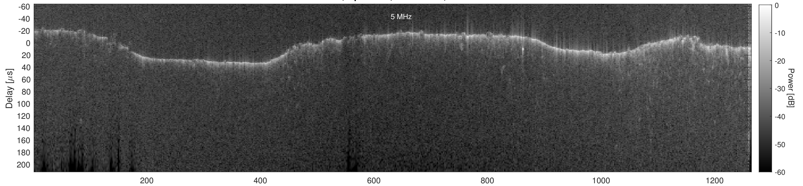
Orbit 18778, Cluttergram
