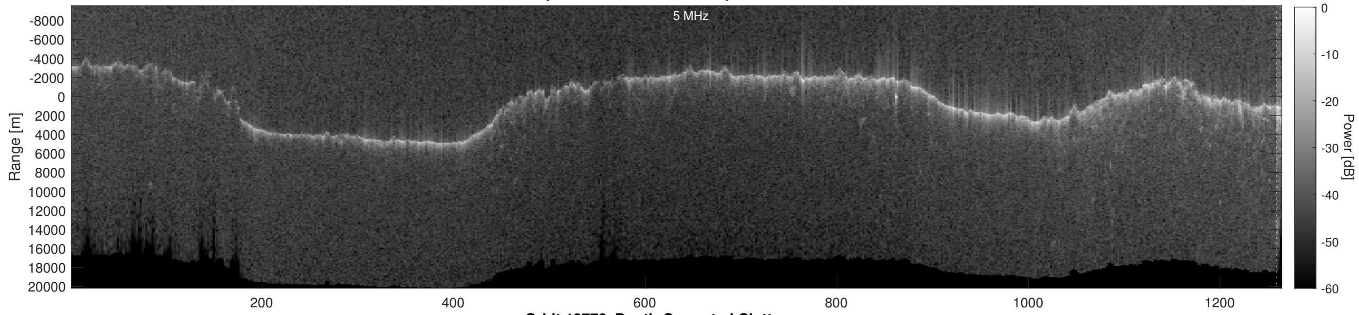
Orbit 18778, Depth-Corrected Cluttergram
