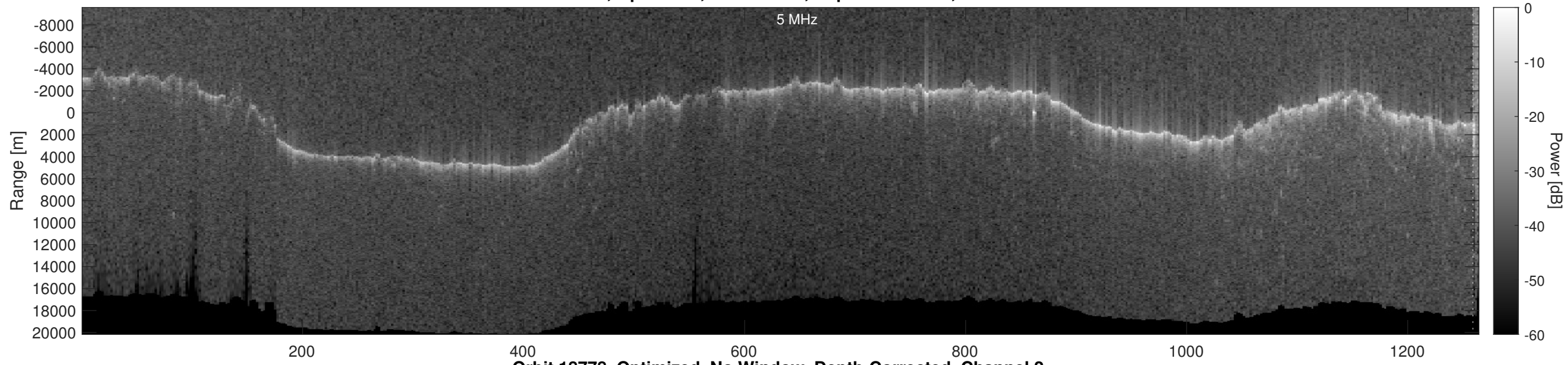
Orbit 18778, Optimized, No Window, Depth-Corrected, Channel 2
