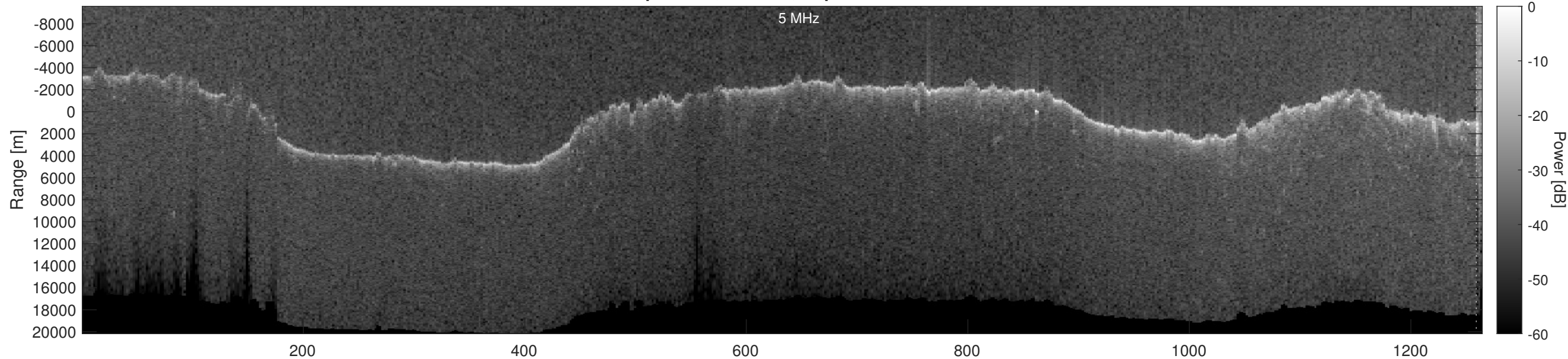
Orbit 18778, Optimized, Window, Depth-Corrected, Channel 2
