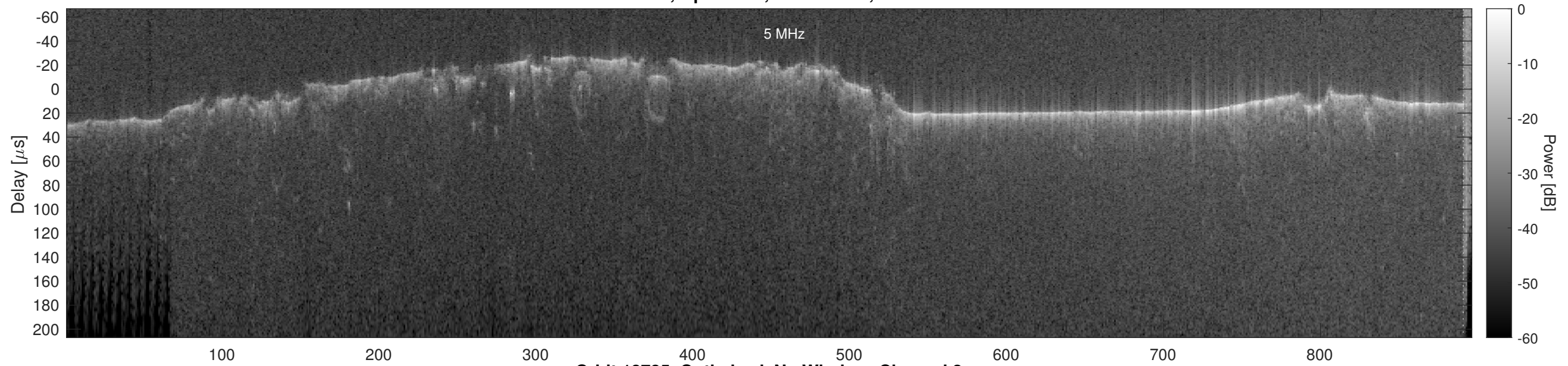
Orbit 18785, Optimized, No Window, Channel 2
