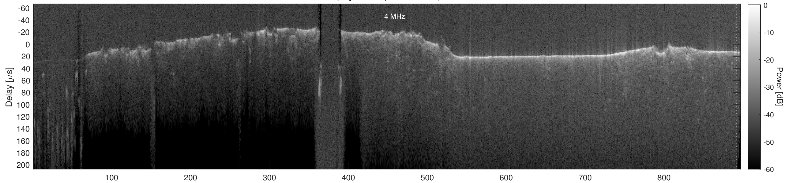
Orbit 18785, Cluttergram
