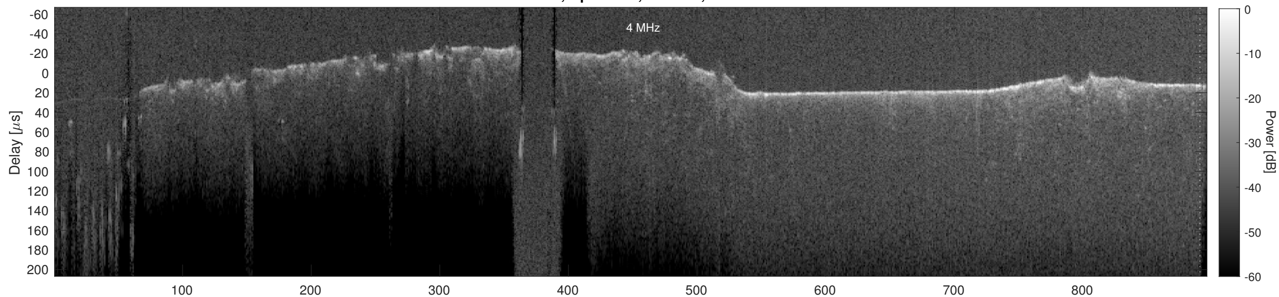
Orbit 18785, Cluttergram
