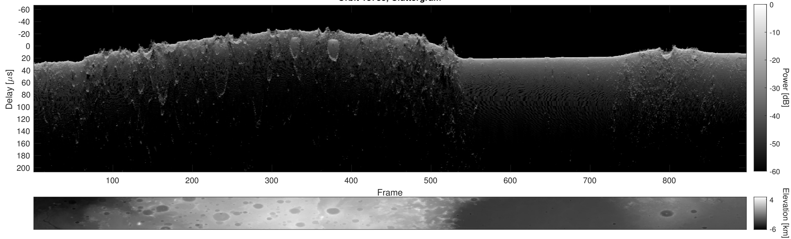
Orbit 18785, Cluttergram
