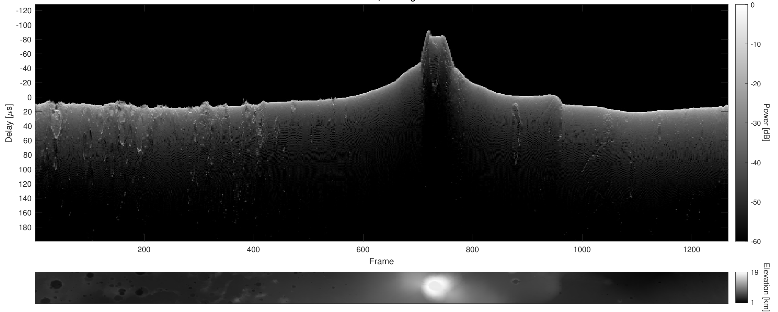
Orbit 18787, Cluttergram
