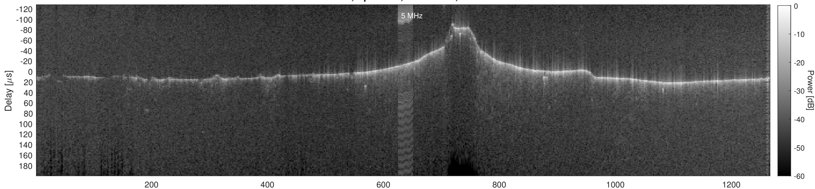
Orbit 18787, Cluttergram
