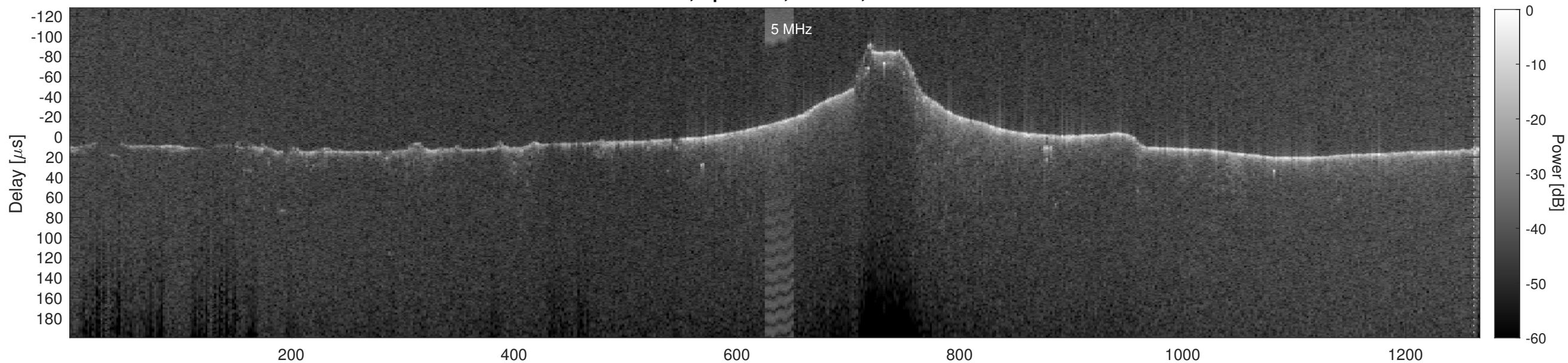
Orbit 18787, Cluttergram
