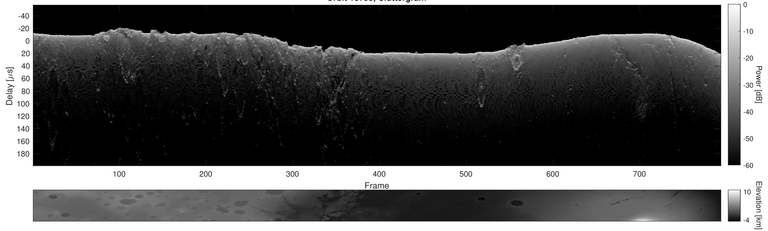
Orbit 18795, Cluttergram
