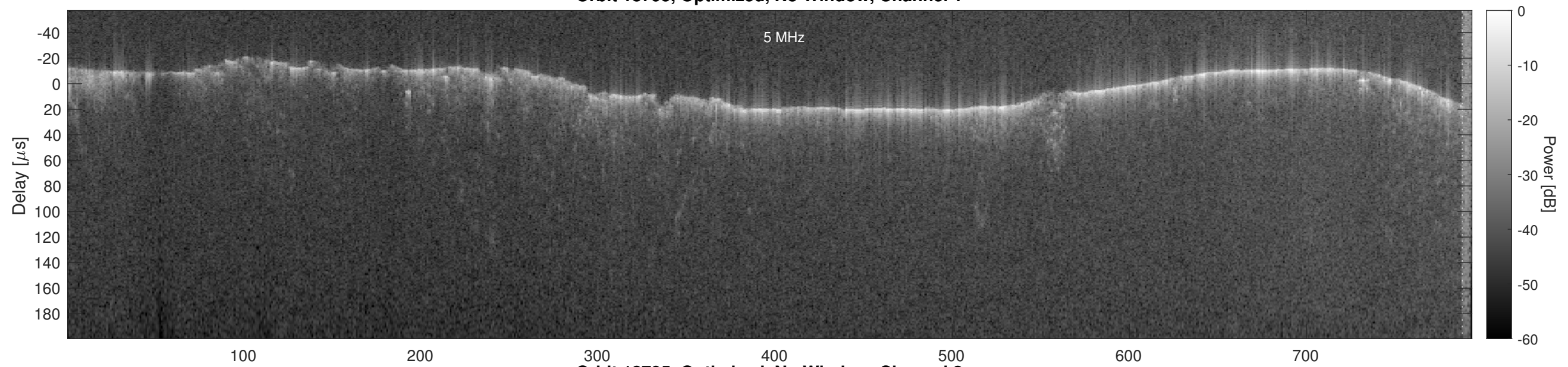
Orbit 18795, Optimized, No Window, Channel 2
