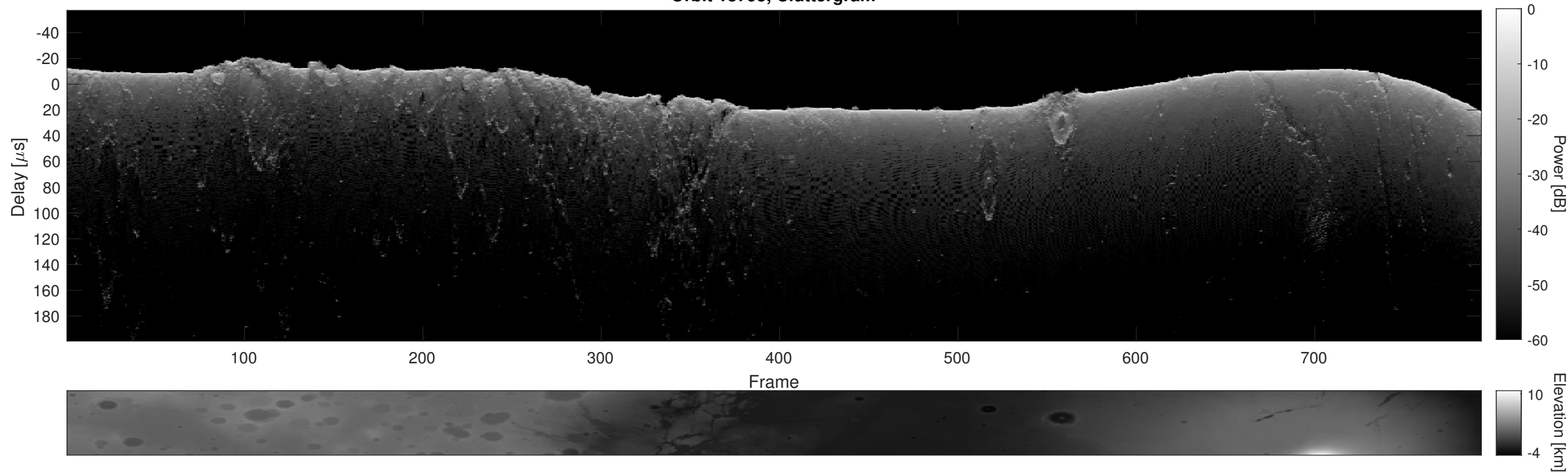
Orbit 18795, Cluttergram
