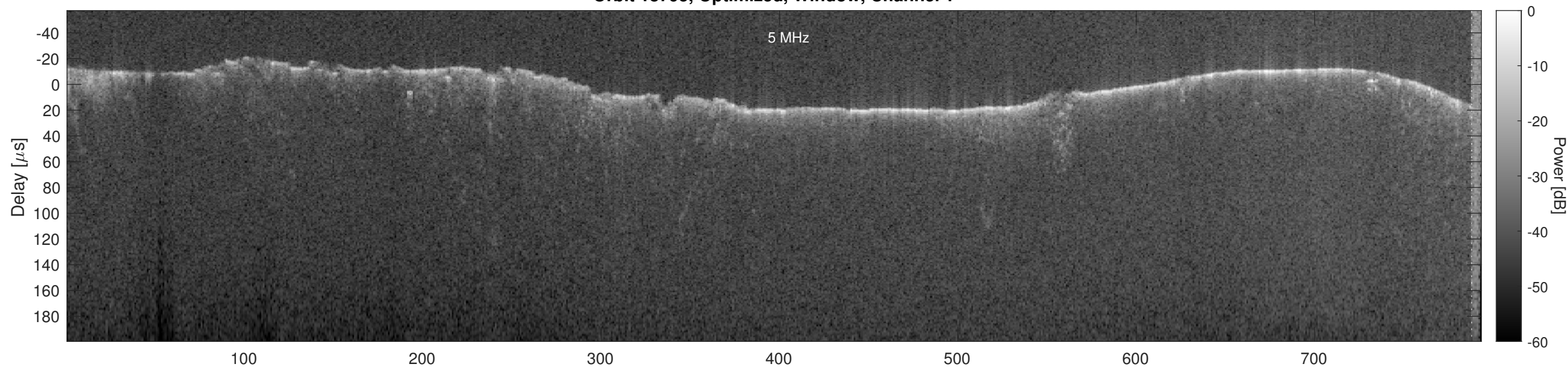
Orbit 18795, Optimized, Window, Channel 2
