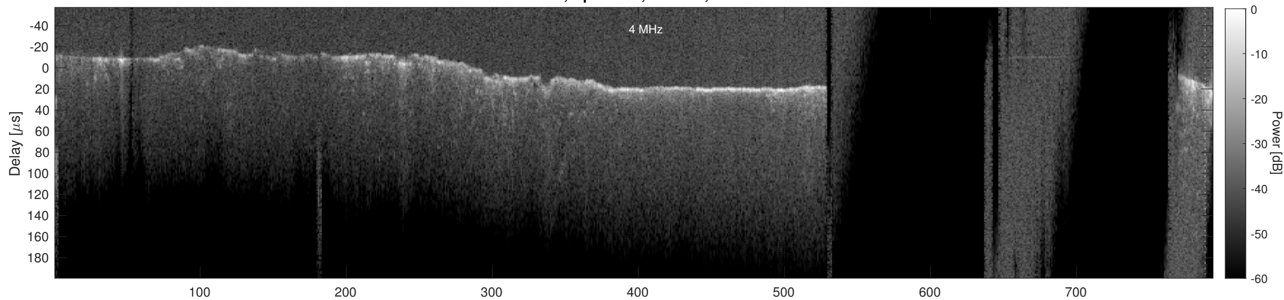
Orbit 18795, Cluttergram
