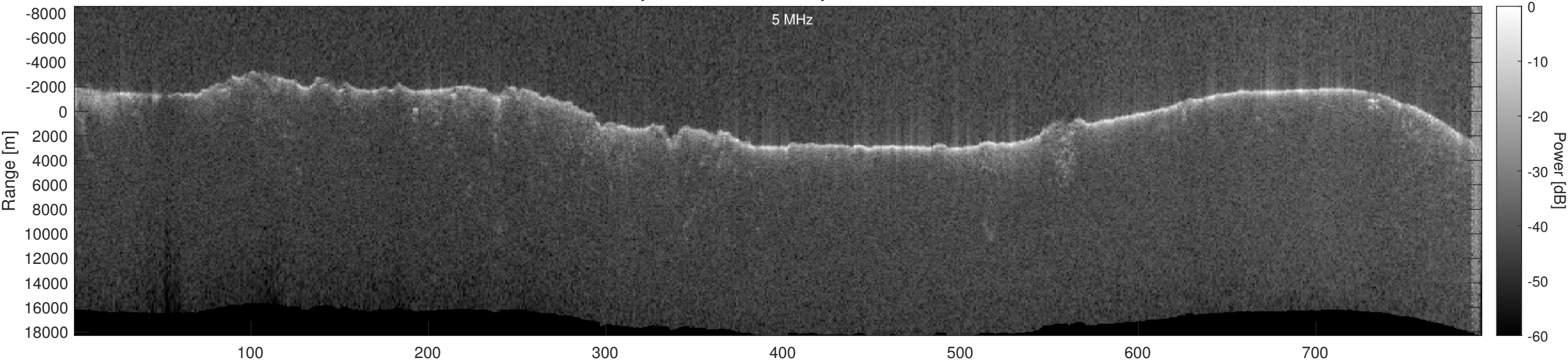
Orbit 18795, Optimized, Window, Depth-Corrected, Channel 2
