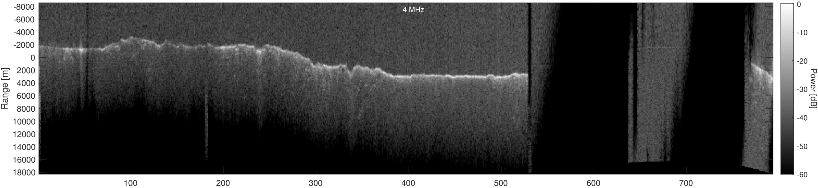
Orbit 18795, Depth-Corrected Cluttergram
