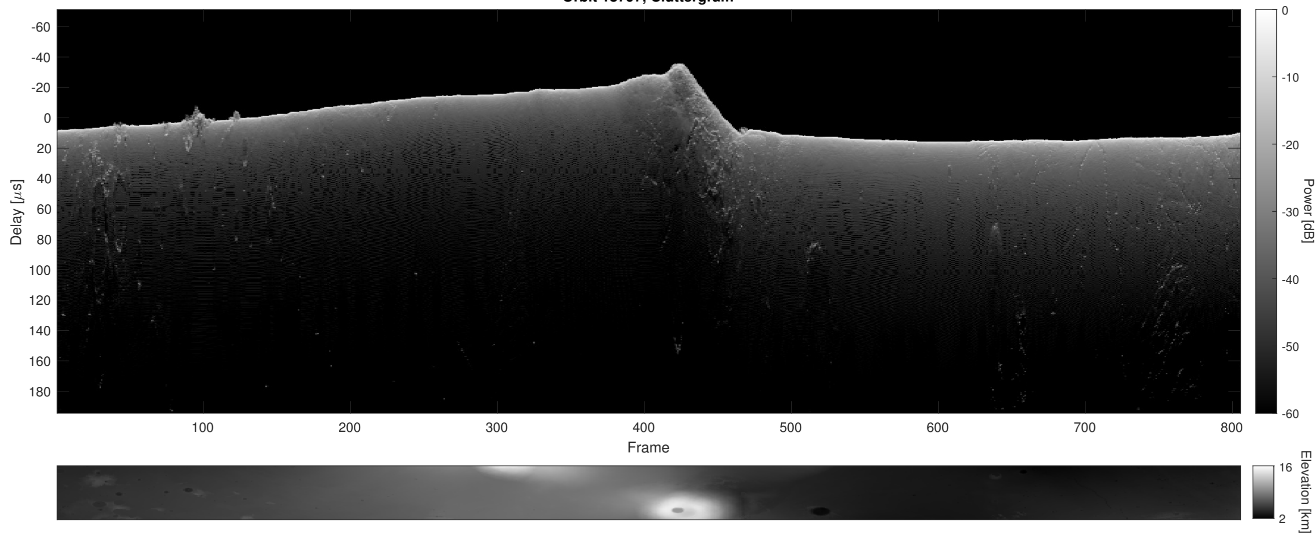
Orbit 18797, Cluttergram
