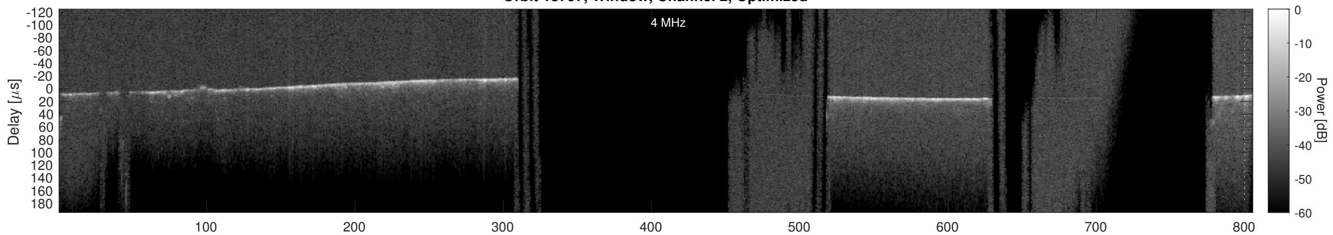
Orbit 18797, Cluttergram
