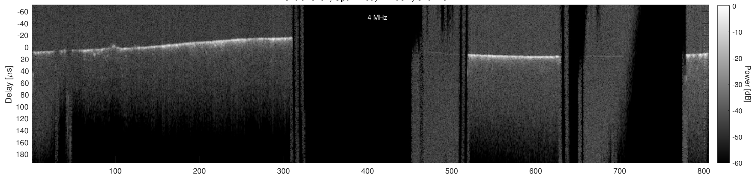
Orbit 18797, Cluttergram
