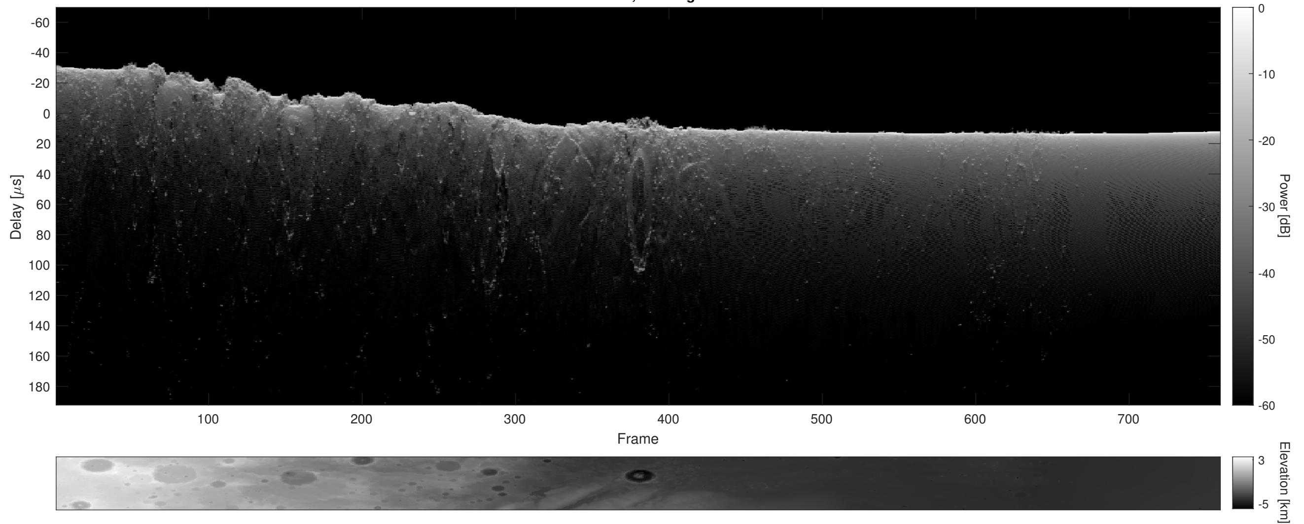
Orbit 18798, Cluttergram
