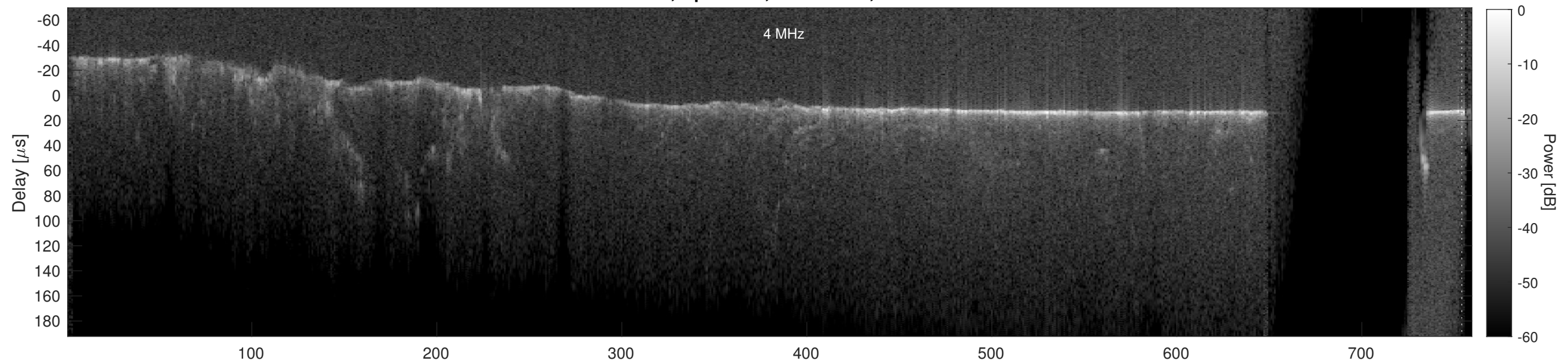
Orbit 18798, Cluttergram
