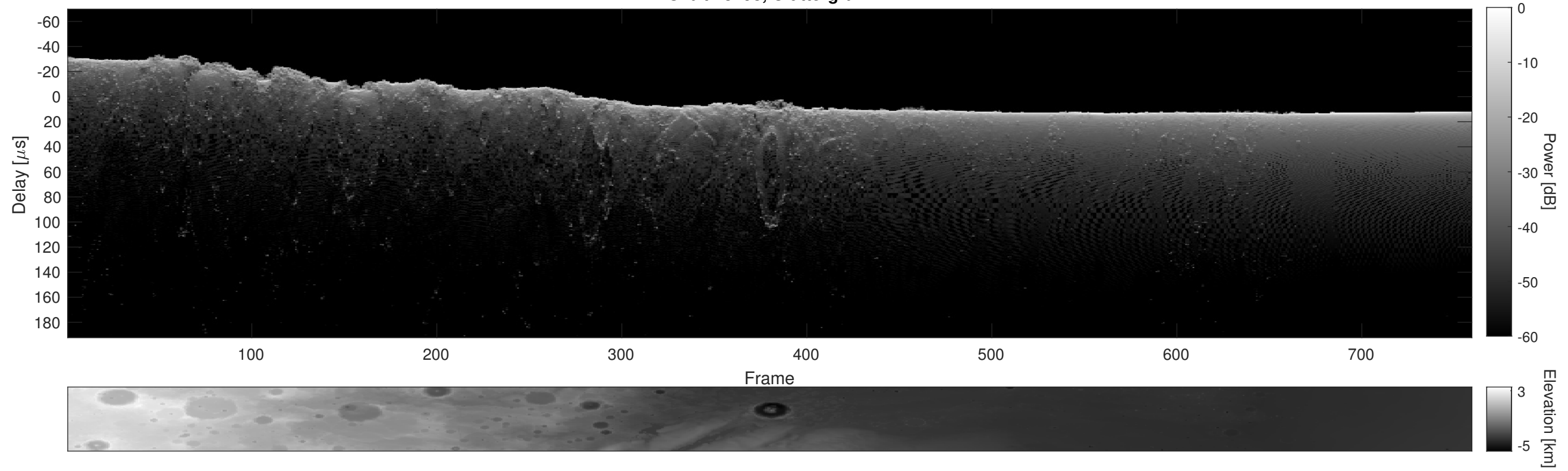
Orbit 18798, Cluttergram
