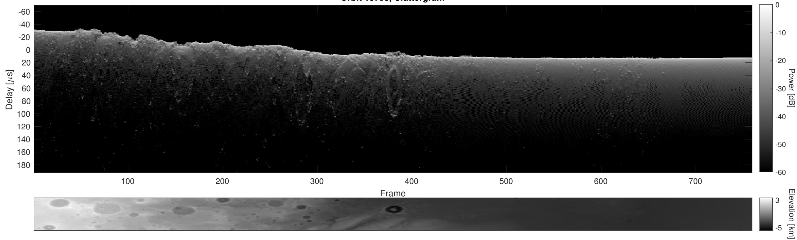
Orbit 18798, Cluttergram
