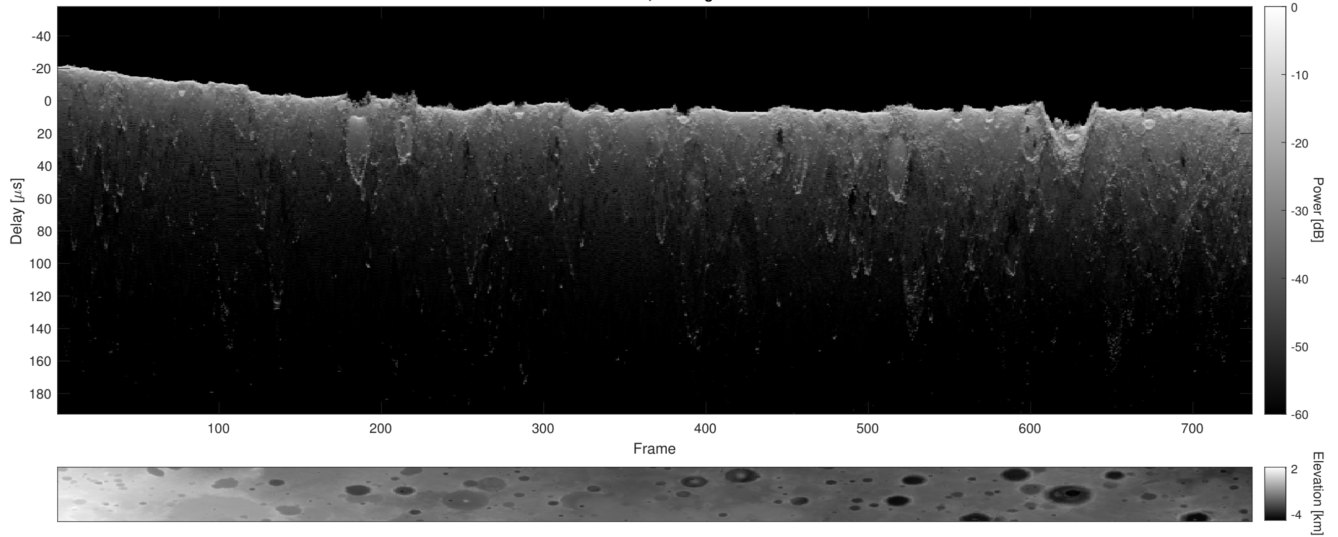
Orbit 18800, Cluttergram
