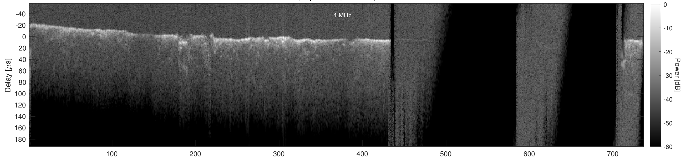
Orbit 18800, Cluttergram
