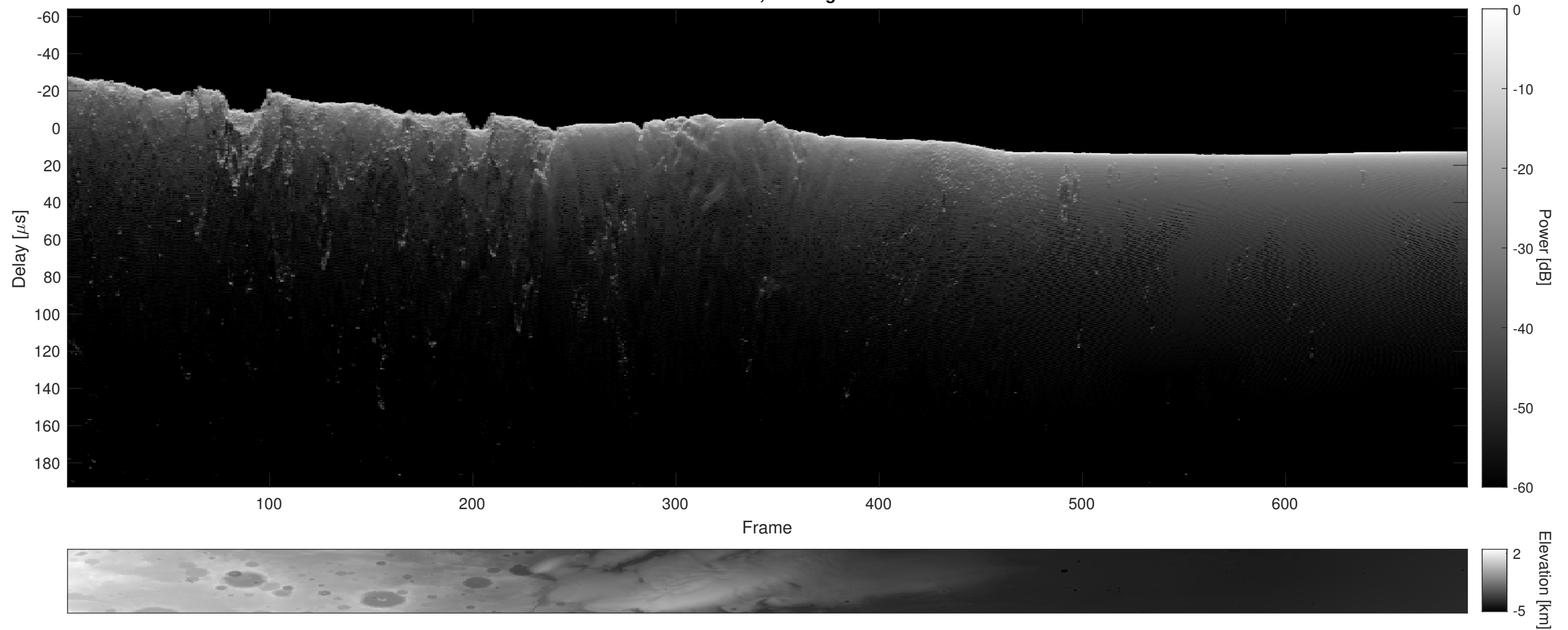
Orbit 18805, Cluttergram
