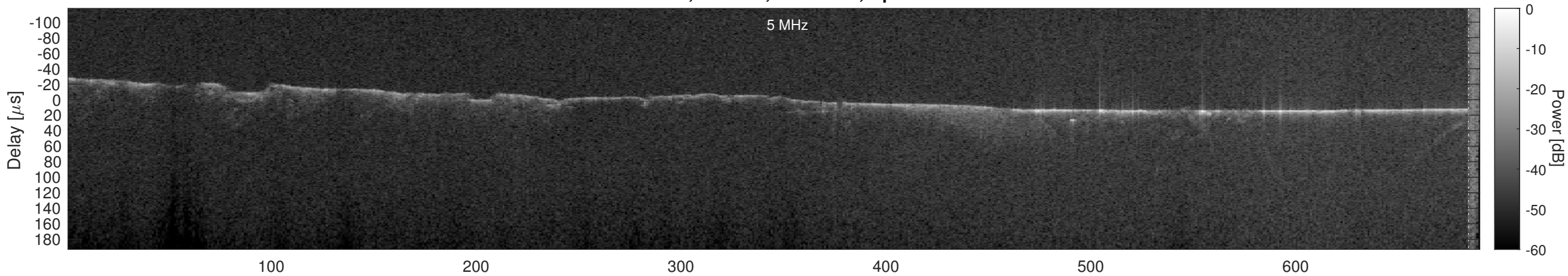
Orbit 18805, Cluttergram
