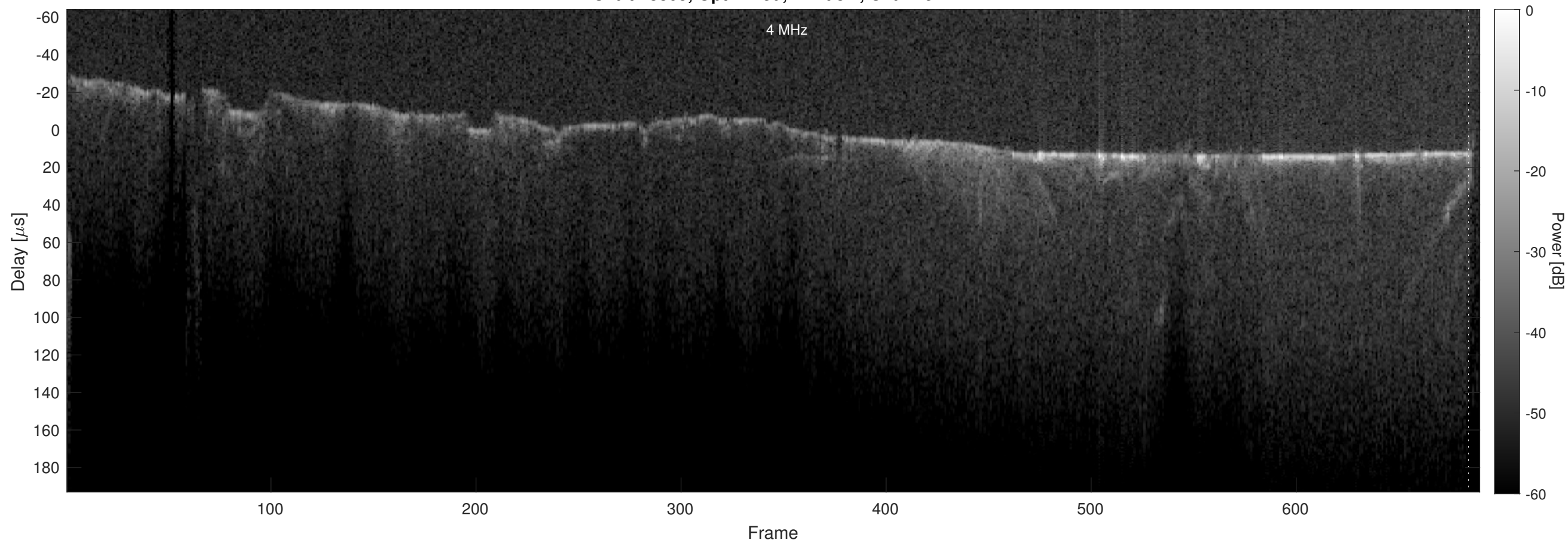
Orbit 18805, Optimized, Window, Channel 2
