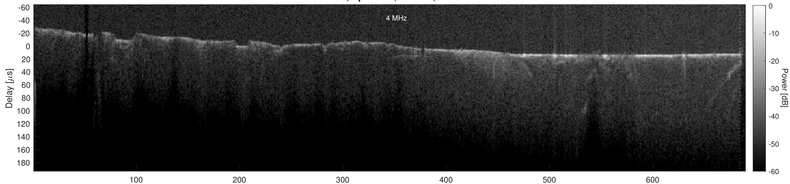
Orbit 18805, Cluttergram
