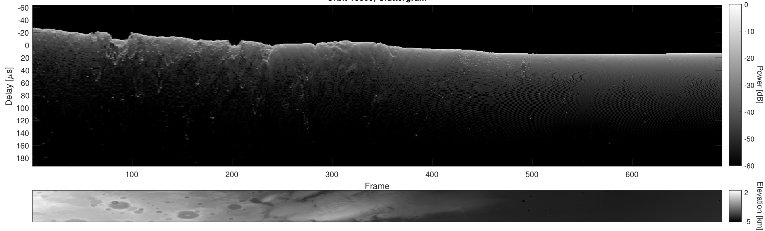
Orbit 18805, Cluttergram
