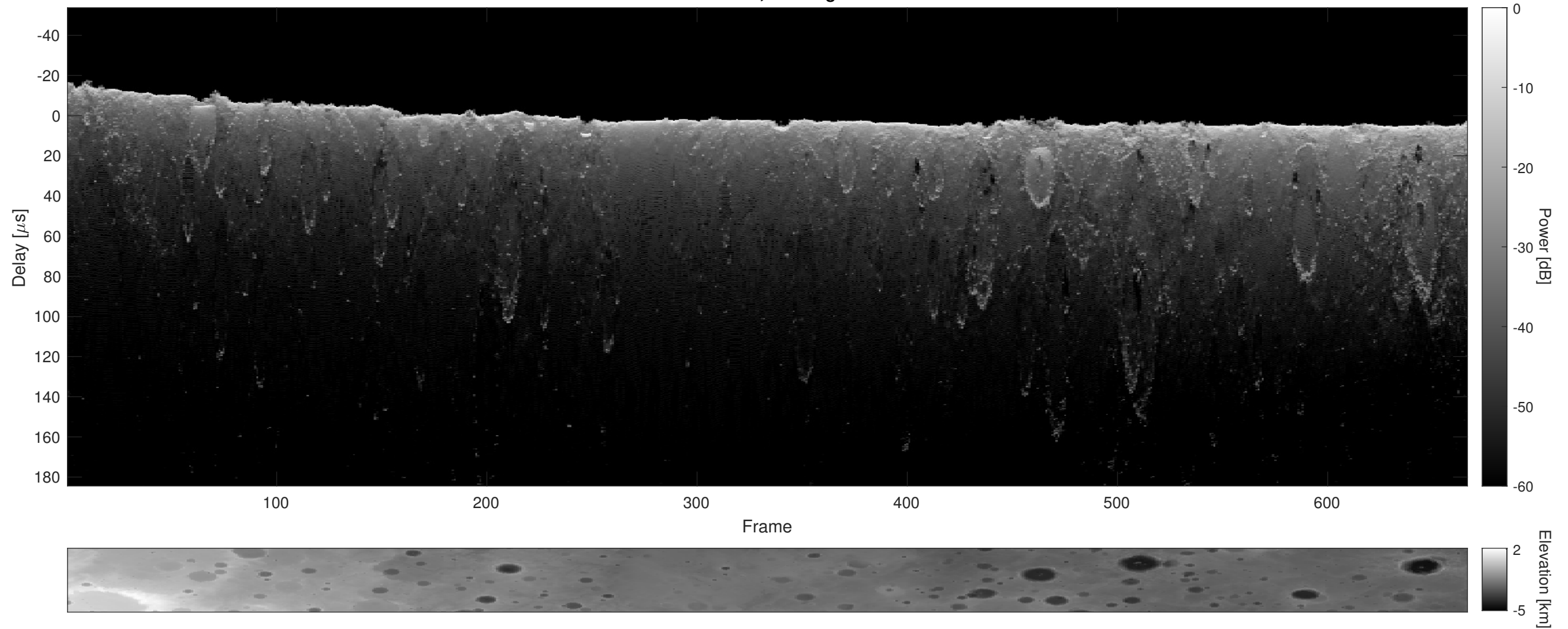
Orbit 18807, Cluttergram
