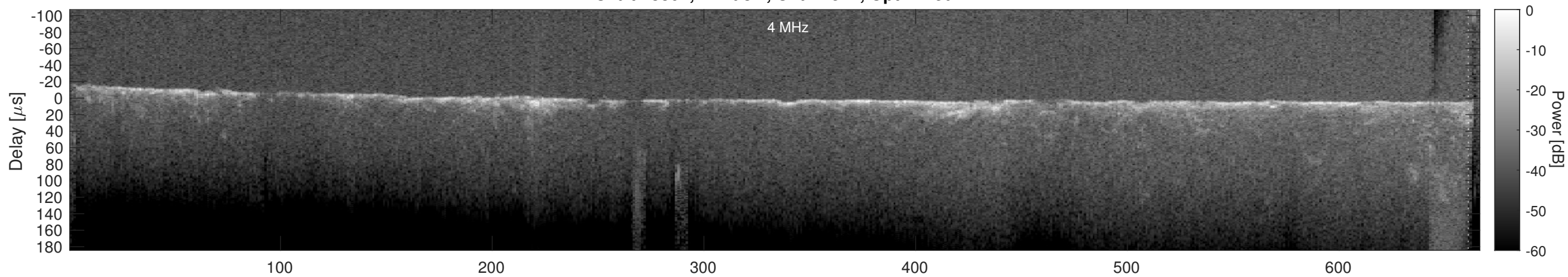
Orbit 18807, Cluttergram
