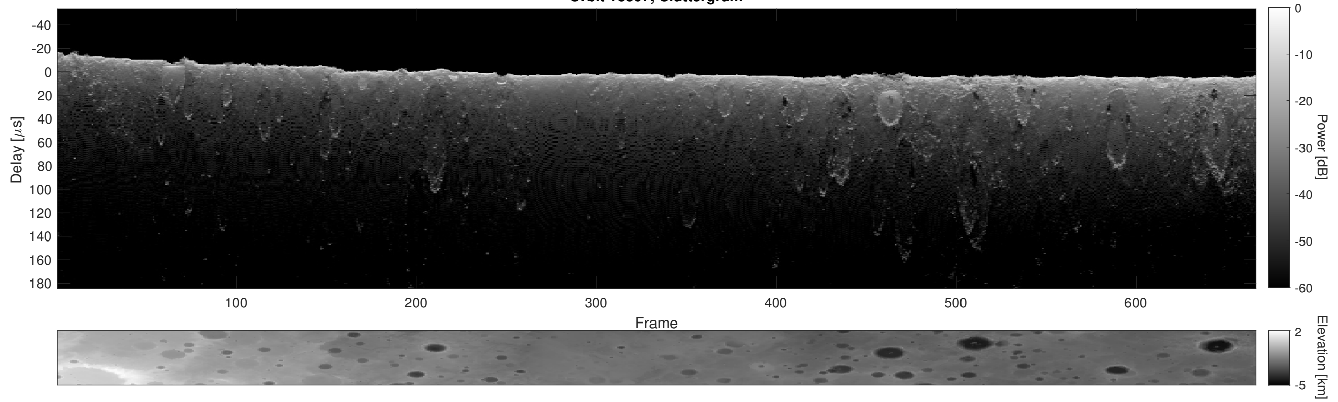
Orbit 18807, Cluttergram
