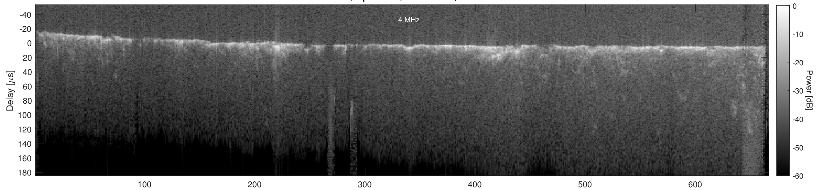
Orbit 18807, Cluttergram
