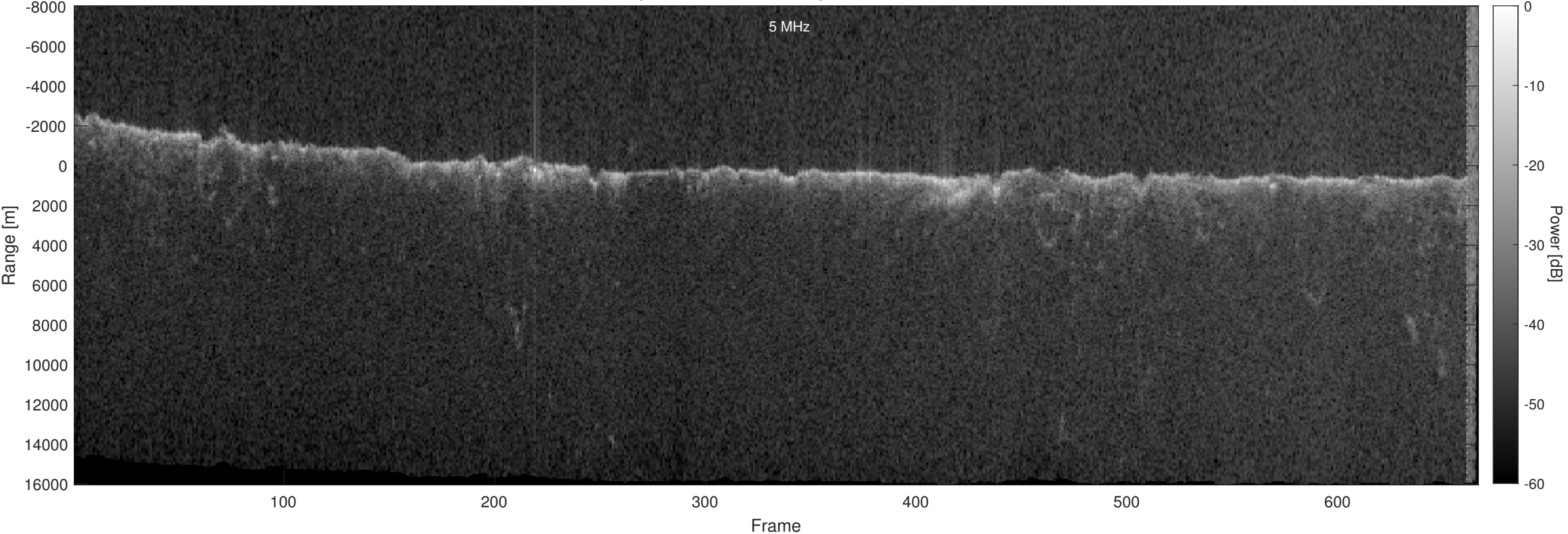
Orbit 18807, Optimized, Window, Depth-Corrected, Channel 2
