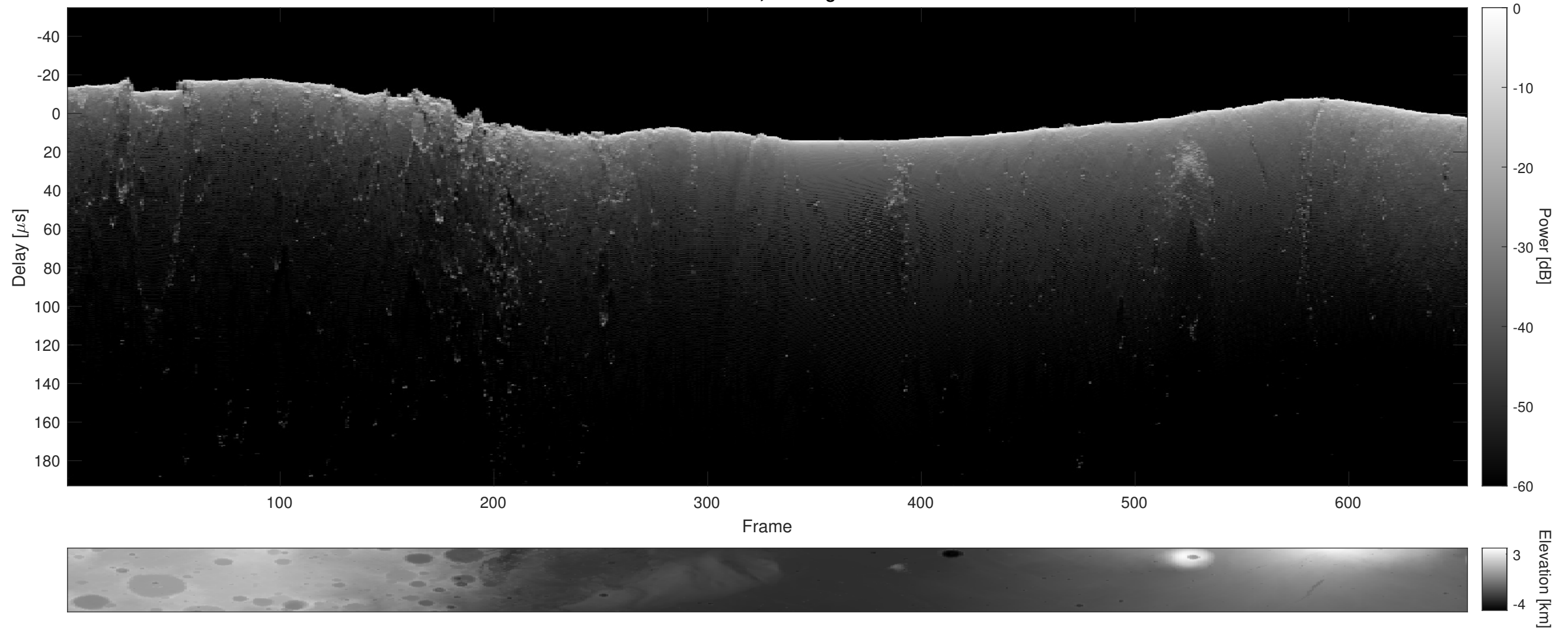
Orbit 18809, Cluttergram
