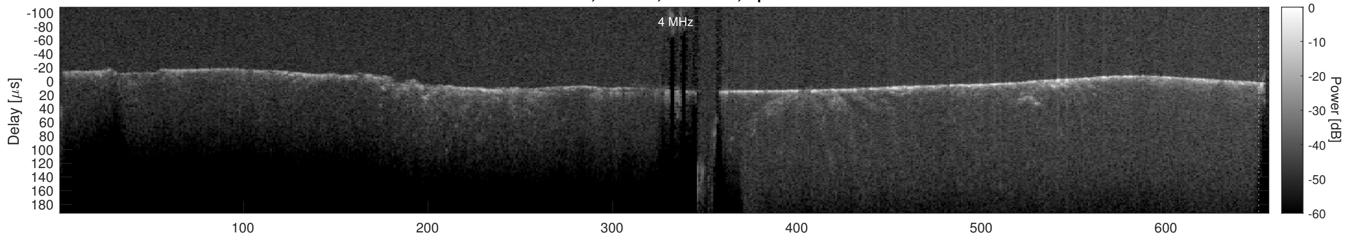
Orbit 18809, Cluttergram
