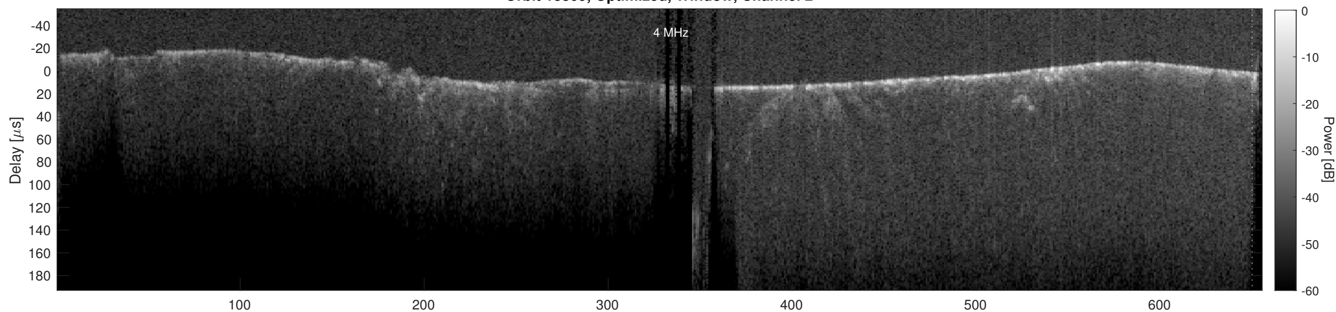
Orbit 18809, Cluttergram
