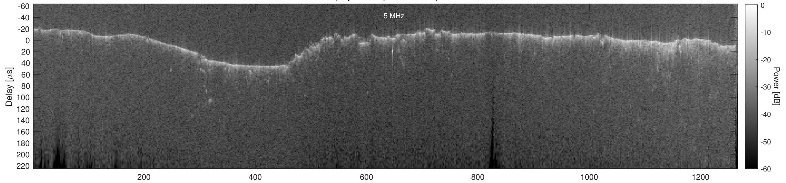
Orbit 18810, Cluttergram
