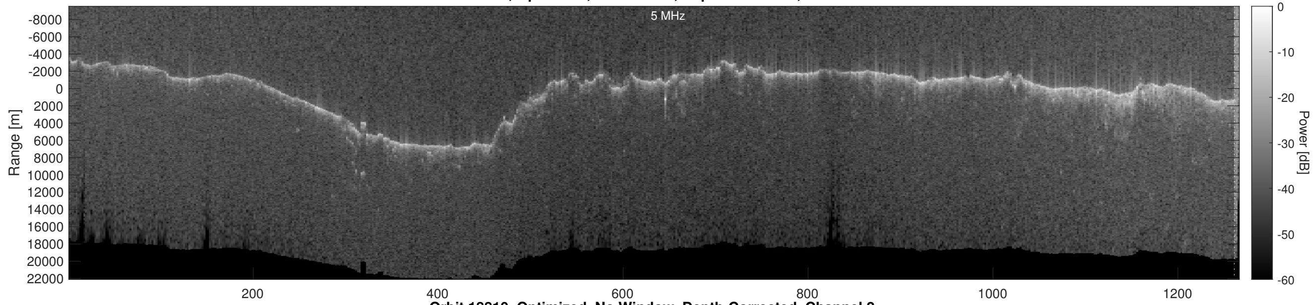
Orbit 18810, Optimized, No Window, Depth-Corrected, Channel 2
