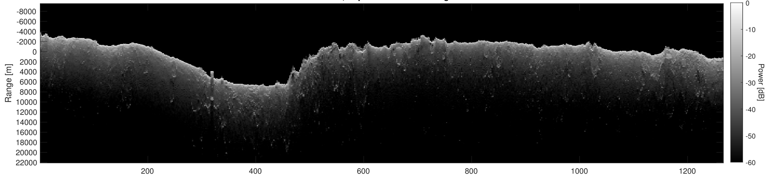
Orbit 18810, Depth-Corrected Cluttergram
