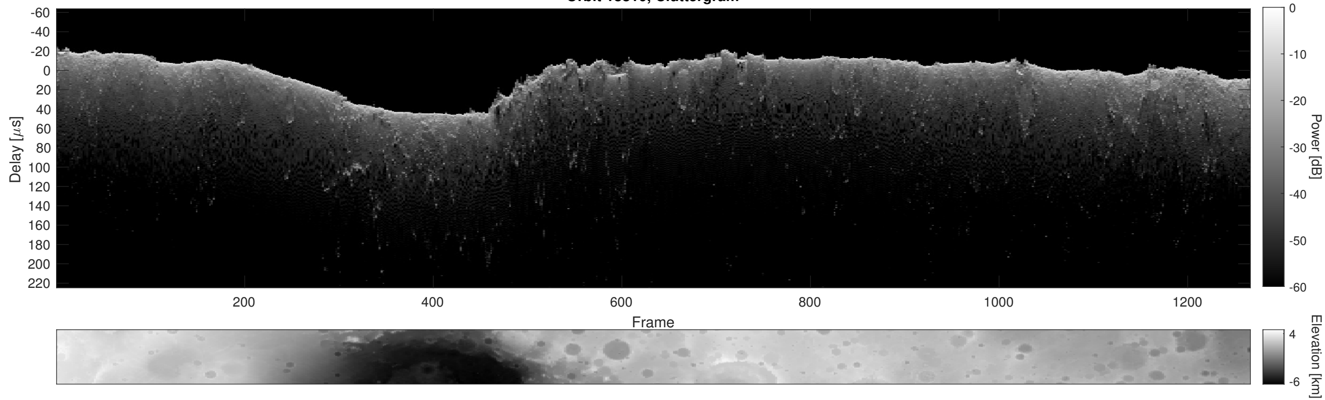
Orbit 18810, Cluttergram
