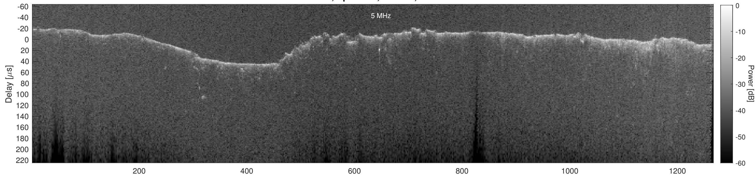
Orbit 18810, Cluttergram
