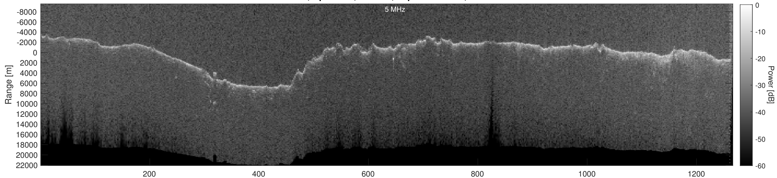
Orbit 18810, Depth-Corrected Cluttergram
