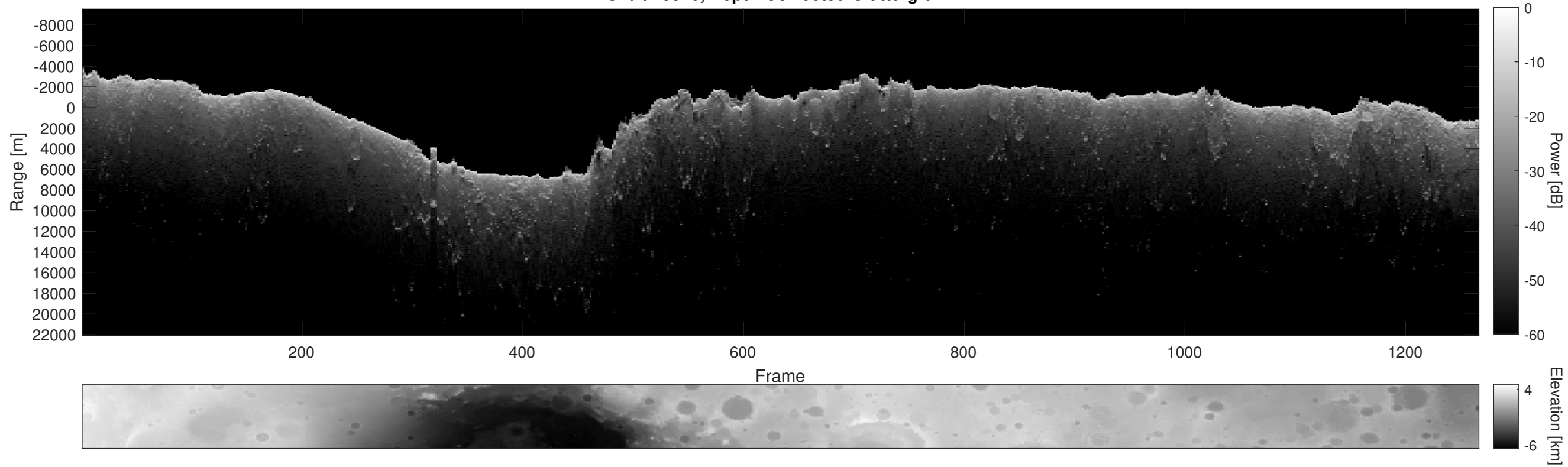
Orbit 18810, Depth-Corrected Cluttergram
