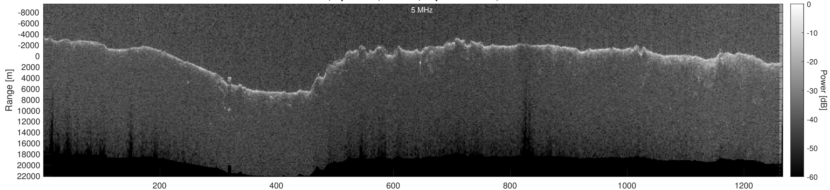
Orbit 18810, Optimized, Window, Depth-Corrected, Channel 2
