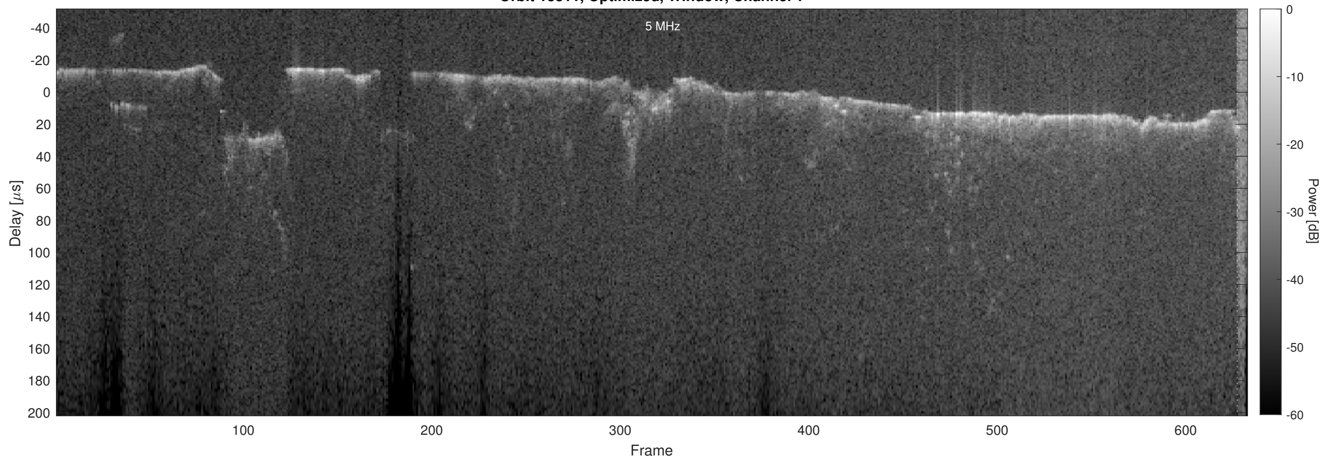
Orbit 18811, Optimized, Window, Channel 2
