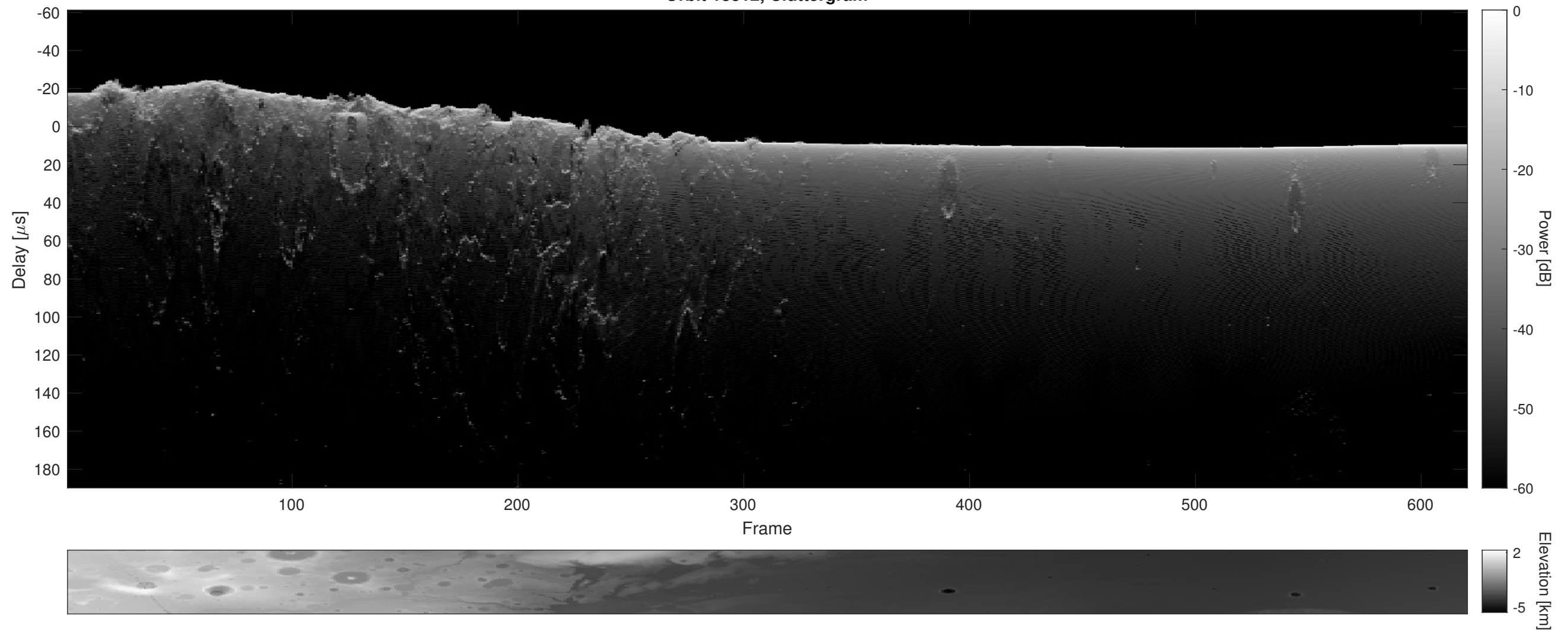
Orbit 18812, Cluttergram
