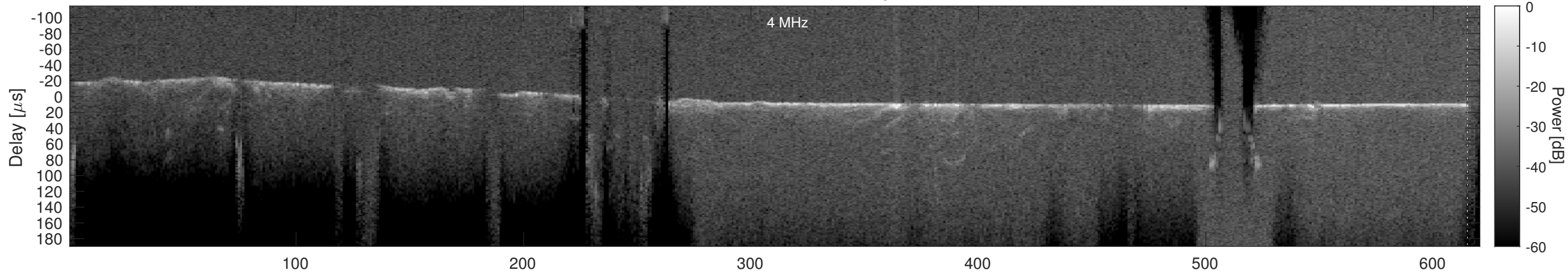
Orbit 18812, Cluttergram
