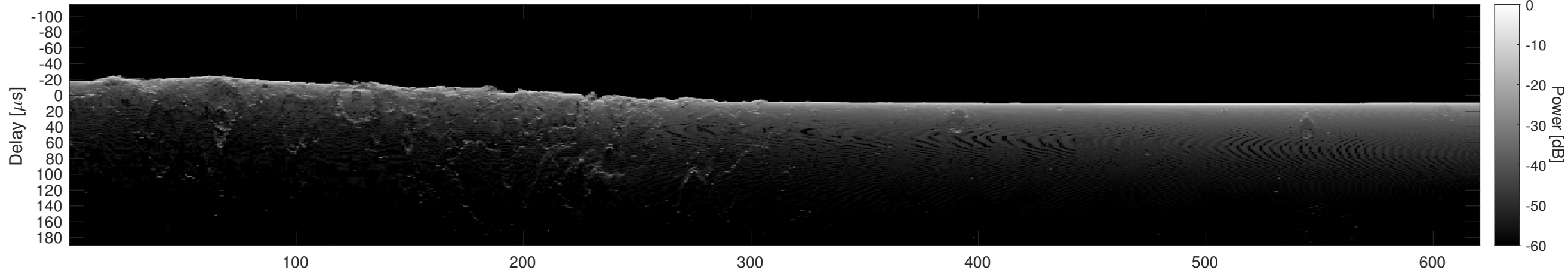
Orbit 18812, Cluttergram
