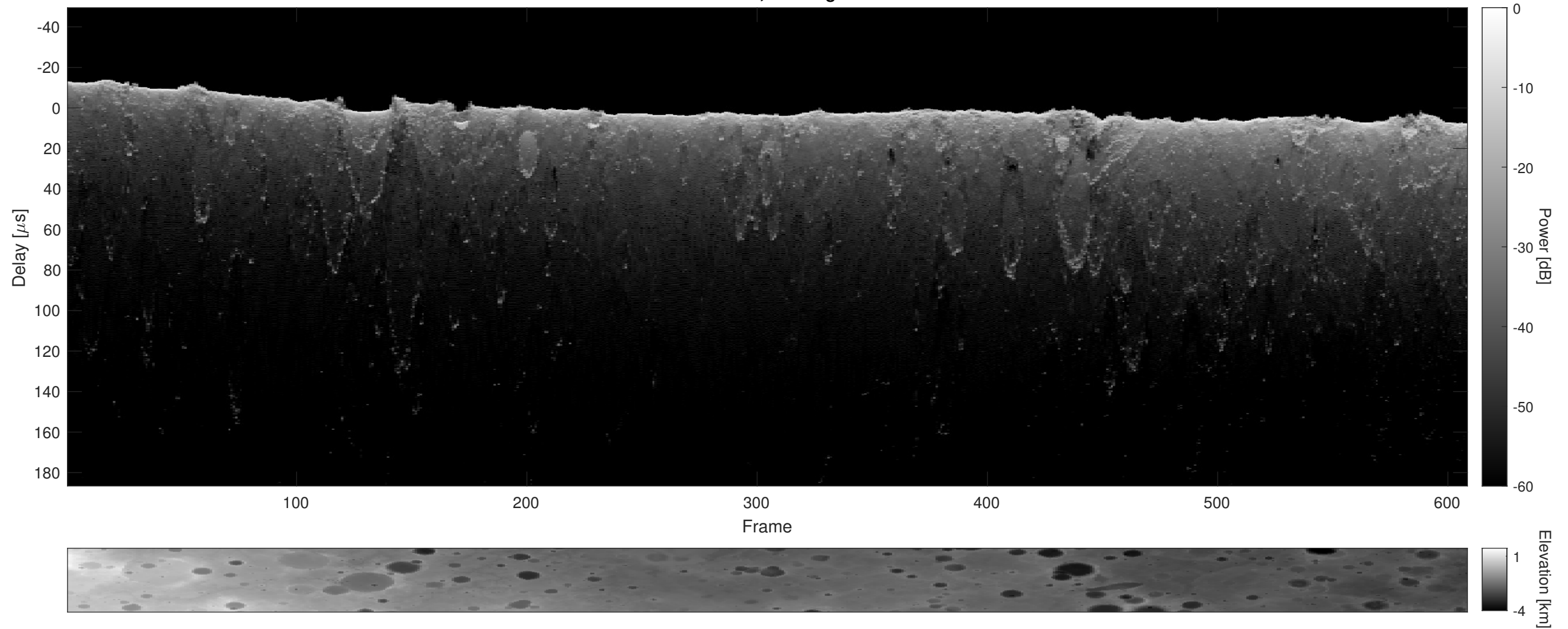
Orbit 18814, Cluttergram
