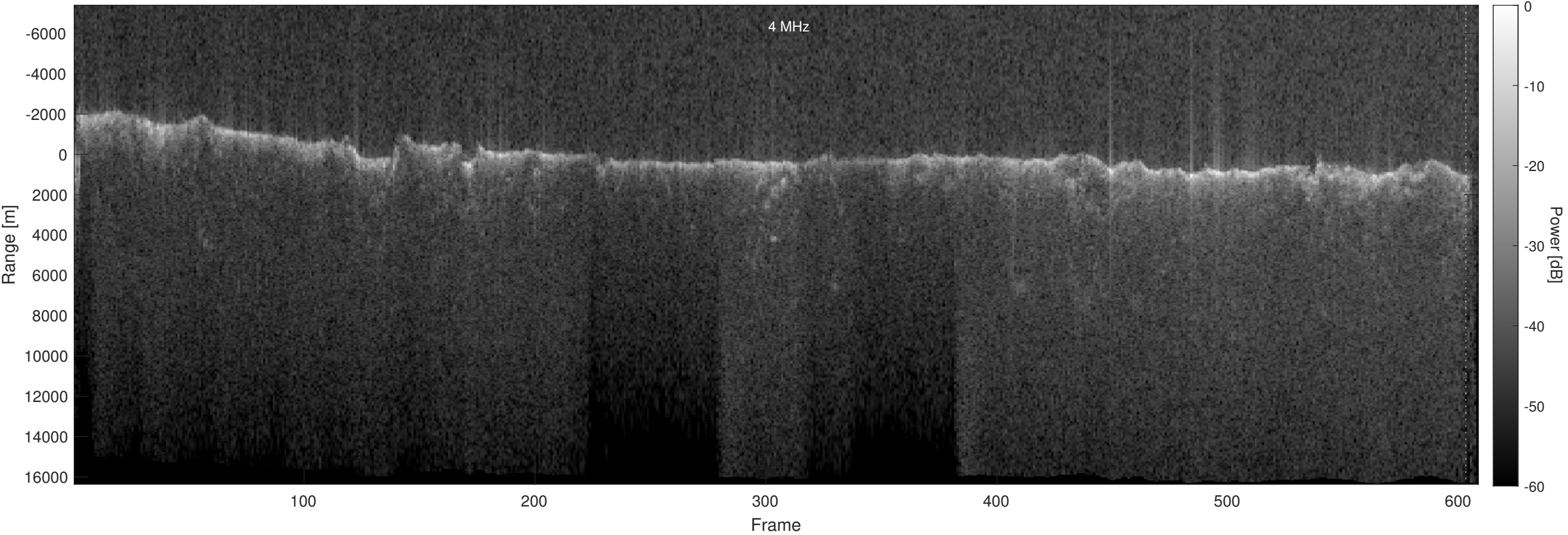
Orbit 18814, Optimized, No Window, Depth-Corrected, Channel 2
